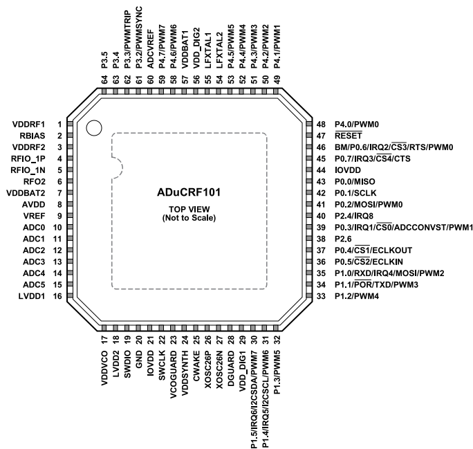
Figure 7. Pin Configuration
