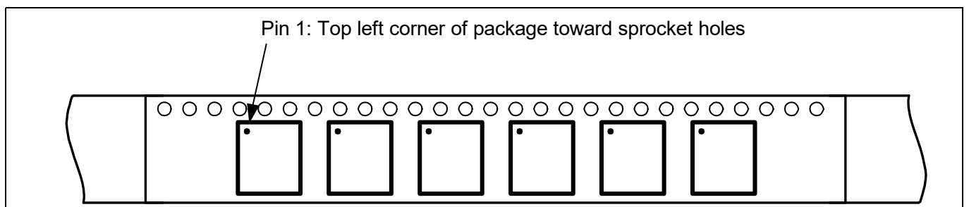
Figure 17 Pin 1 orientation
