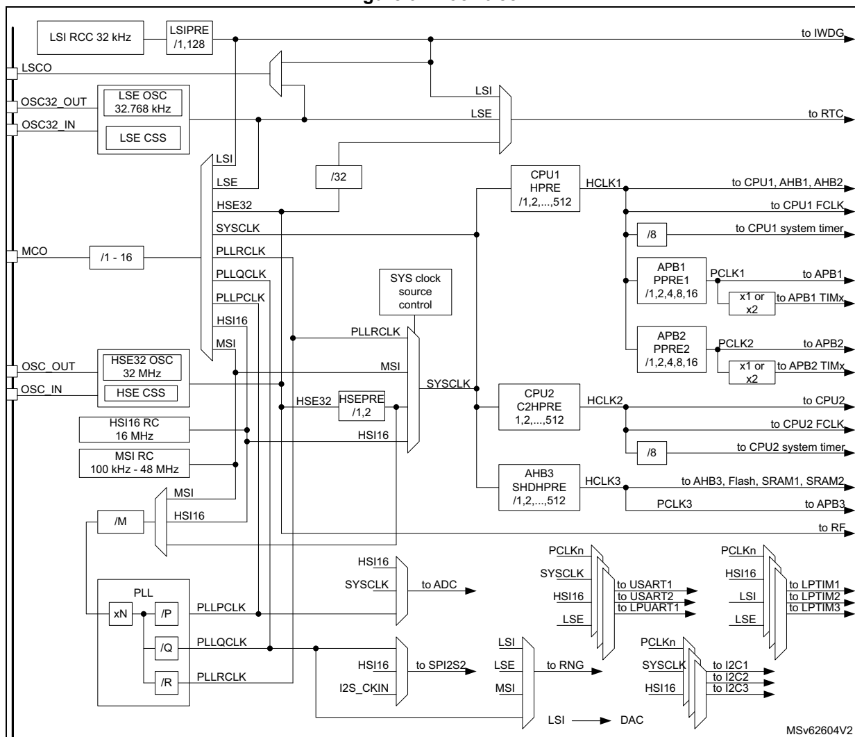
Figure 9. Clock tree
