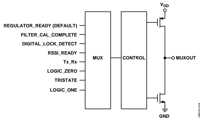
Figure 36. MUXOUT Circuit
