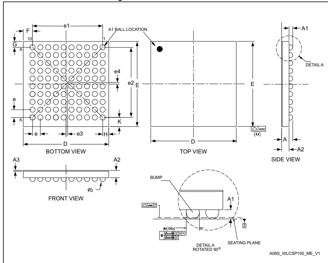
Figure 40. WLCSP100 outline
