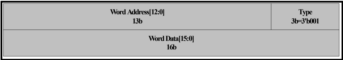
Figure 6-1. Shadow RAM Word Write Command
