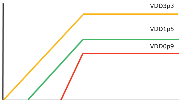
Figure 12-23. Power Sequencing Guideline
