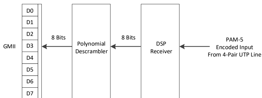
Figure 3-20. Transmit/Receive Flow
