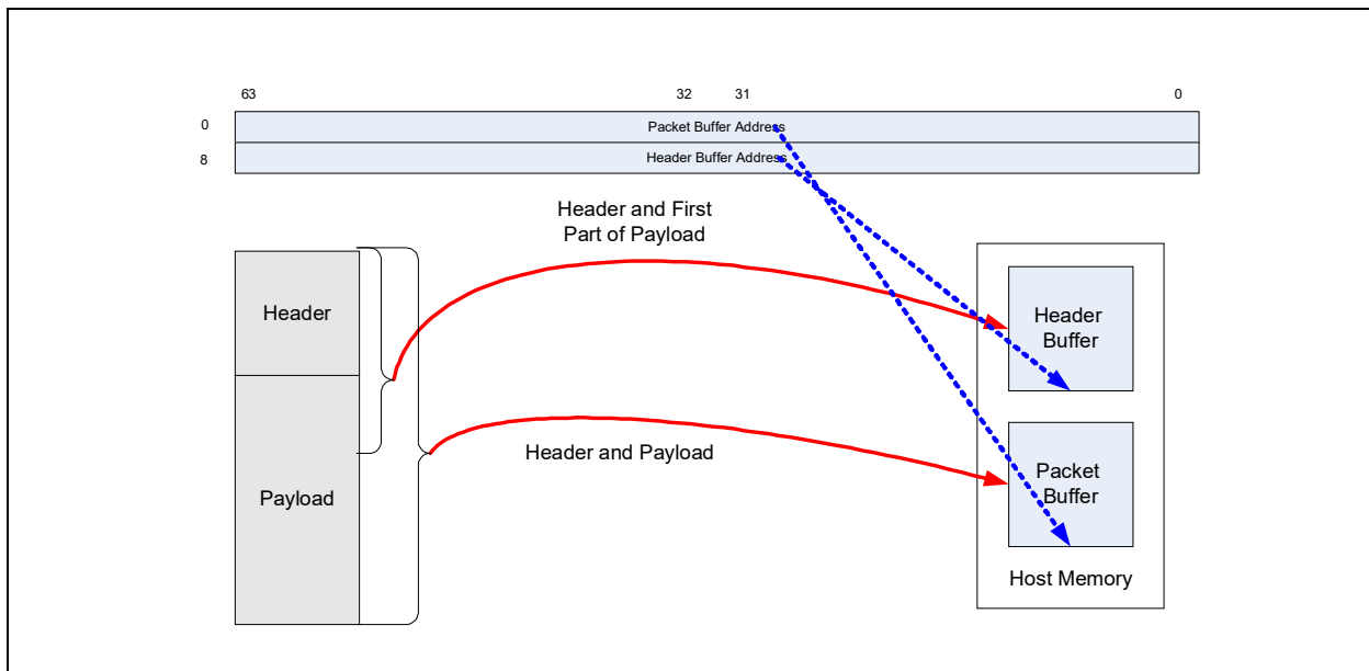
Figure 7-9. Header Replication
