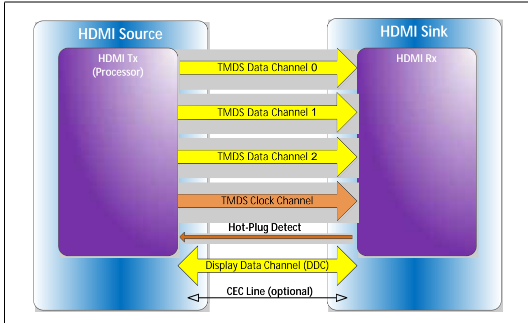
Figure 2-7. HDMI * Overview
