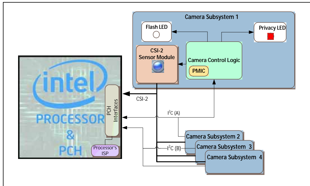
Figure 3-2. Processor Camera System
