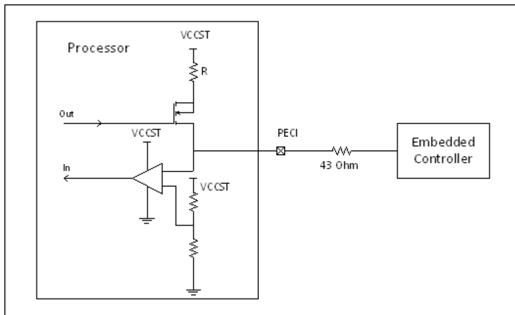
Figure 2-9. Example for PECEC Connection
