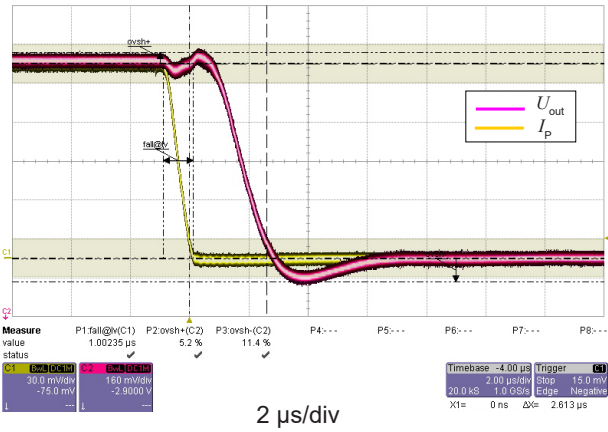
Figure 8: Step response
