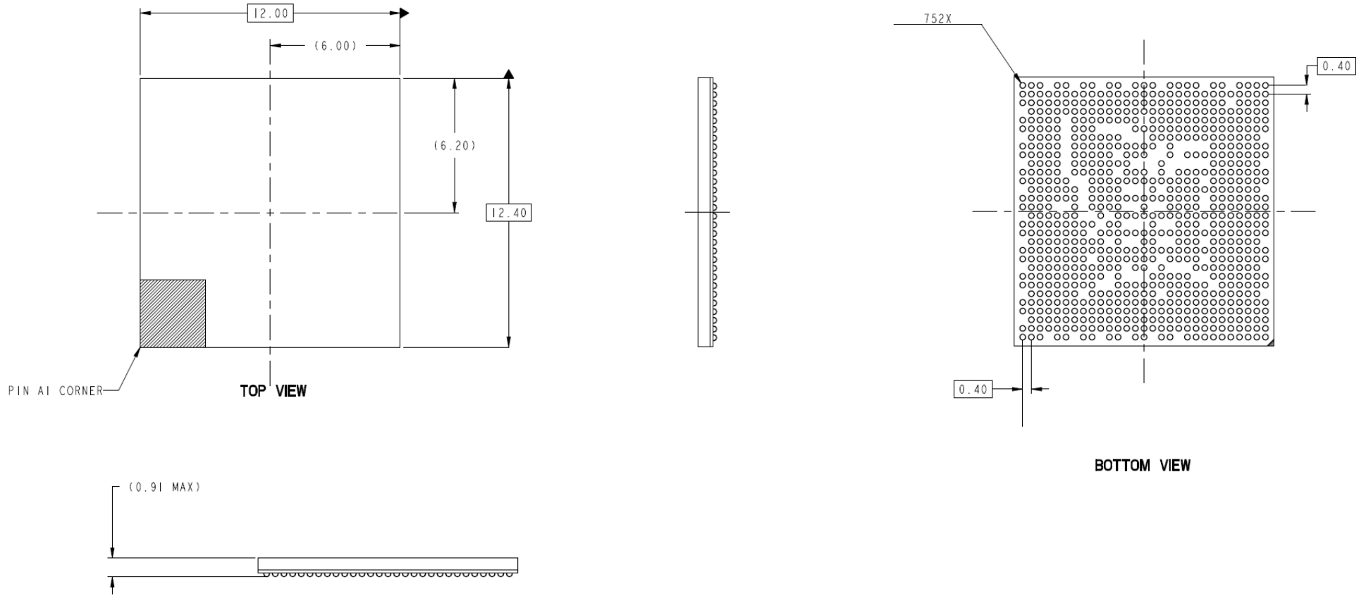
Figure 4-1 NSP752 (12.0 × 12.4 × 0.91 mm) outline drawing
