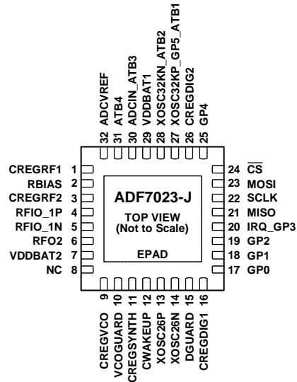
Figure 4. Pin Configuration
