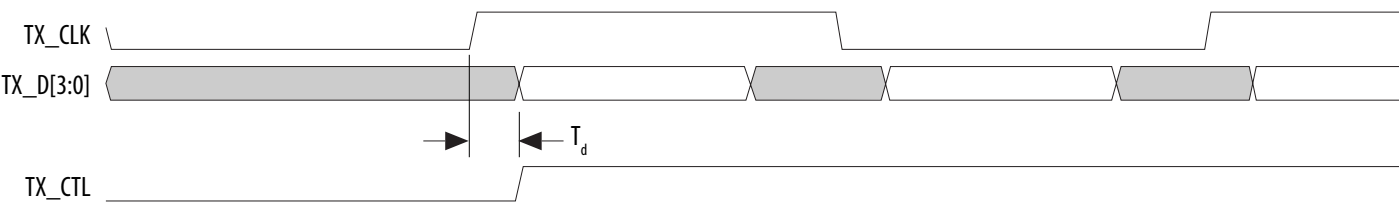
Figure 11. RGMII TX Timing Diagram
