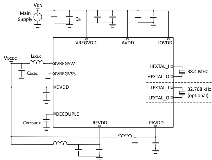
Figure 5.2. EFR32MG22E Typical Application Circuit: DCDC Configuration, PAVDD and RFVDD from DCDC Output, AVDD and IOVDD from Main Supply
