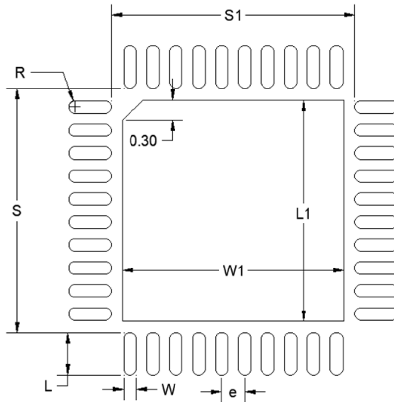
Figure 8.2. QFN40 PCB Land Pattern Drawing
