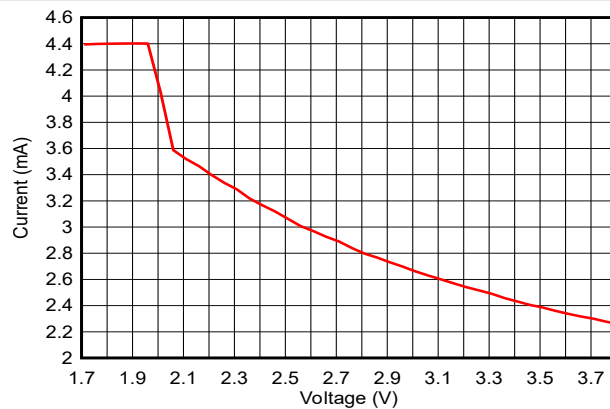
Figure 7-6. Active Mode (MCU) Current vs. Supply Voltage ( V_{DDS} ) (Running CoreMark)
