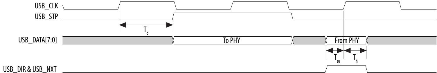
Figure 10. USB Timing Diagram
