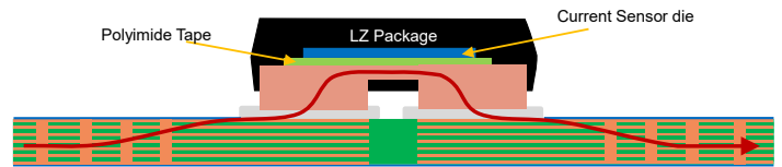
Figure 14: Vias Not Placed Under Copper Pads, LZ Package
