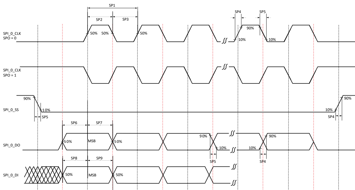
Figure 30-2. SPI Timing for a Single Frame Transfer in Motorola Mode (SPH = 1)
