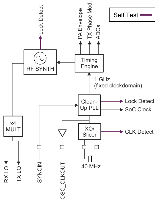
Figure 9-3. Clock Subsystem
