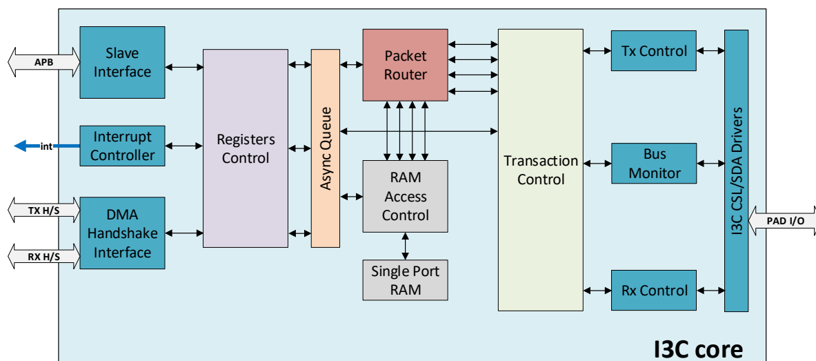
Figure 78: I3C Controller Block Diagram
