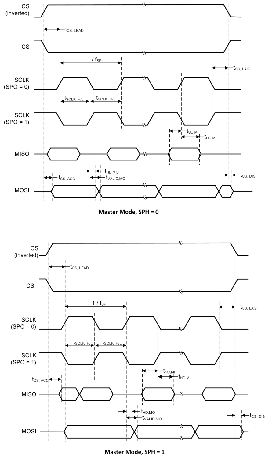
Figure 8-1. SPI Master Mode Timing
