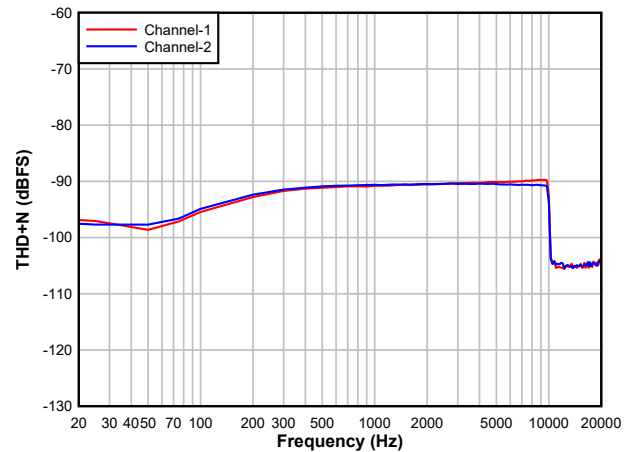
Figure 6-28. DAC THD+N Level vs Frequency
