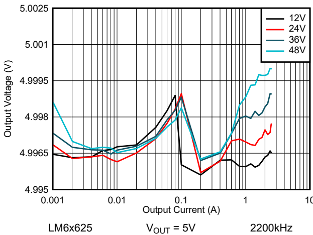
Figure 8-21. LM6x625 Line and Load Regulation - Auto Mode
