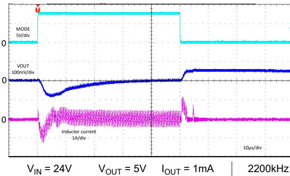
Figure 8-71. MODE Change Transient
