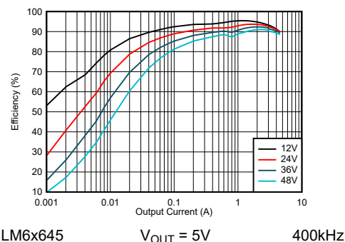
Figure 3-1. LM6x645 Efficiency - Auto Mode
