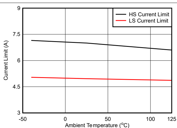
Figure 6-8. 4.5A Current Limit
