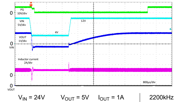
Figure 8-72. Dropout Transient and Recovery
