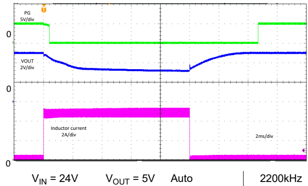
Figure 8-70. Current Limit Transient
