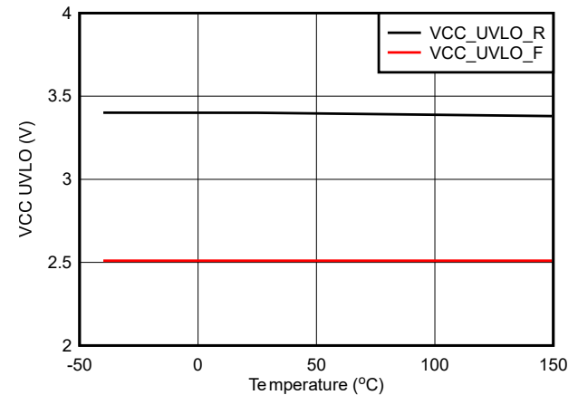
Figure 6-4. V_{CC} UVLO
