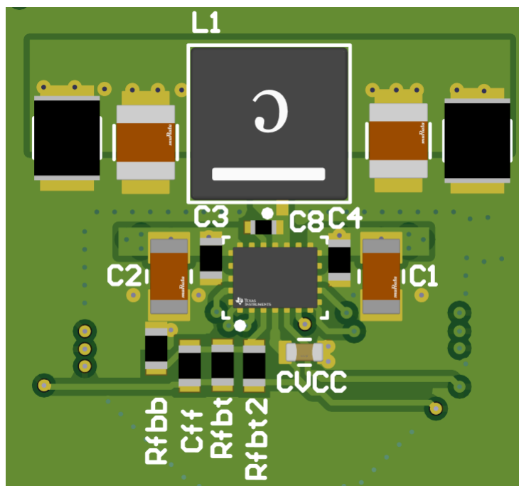
Figure 8-79. PCB Image
