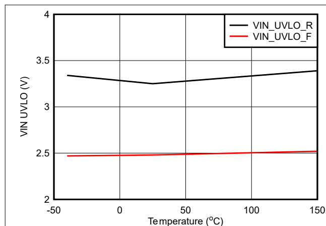
Figure 6-7. V_{IN} UVLO
