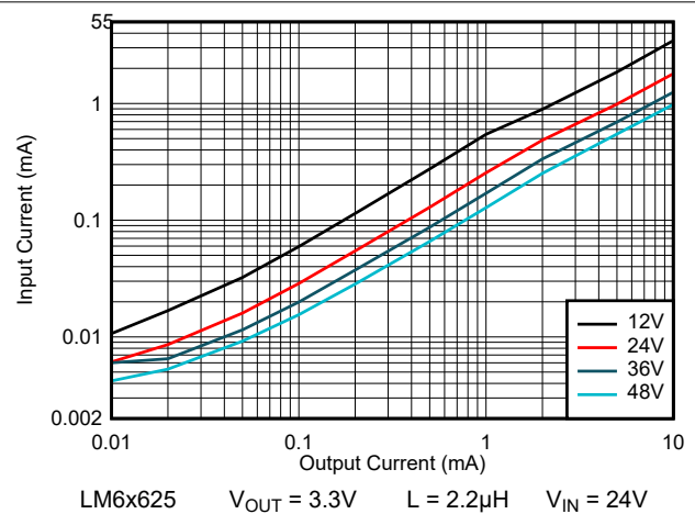
Figure 8-42. Input Supply Current - Auto Mode
