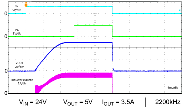
Figure 8-68. Start-up/Shutdown - FPWM
