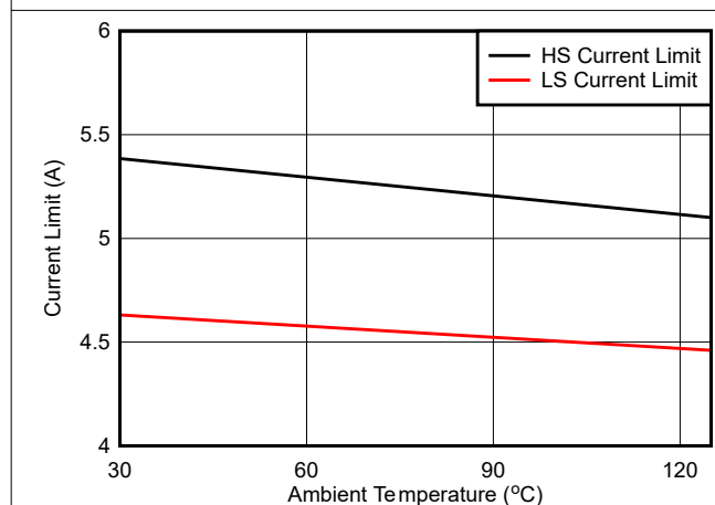
Figure 6-9. 3.5A Current Limit
