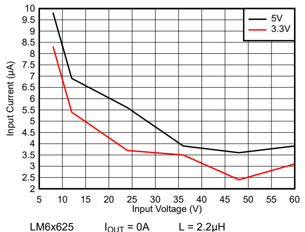
Figure 8-48. No Load Input Supply Current - Auto Mode
