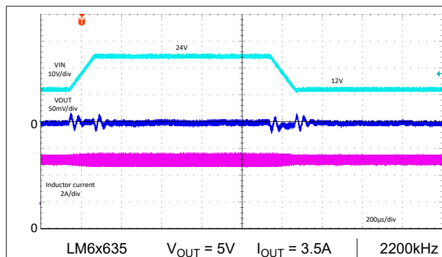
Figure 8-73. Line Transient - Auto
