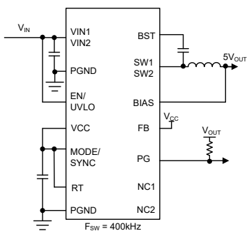
Simplified Schematic
