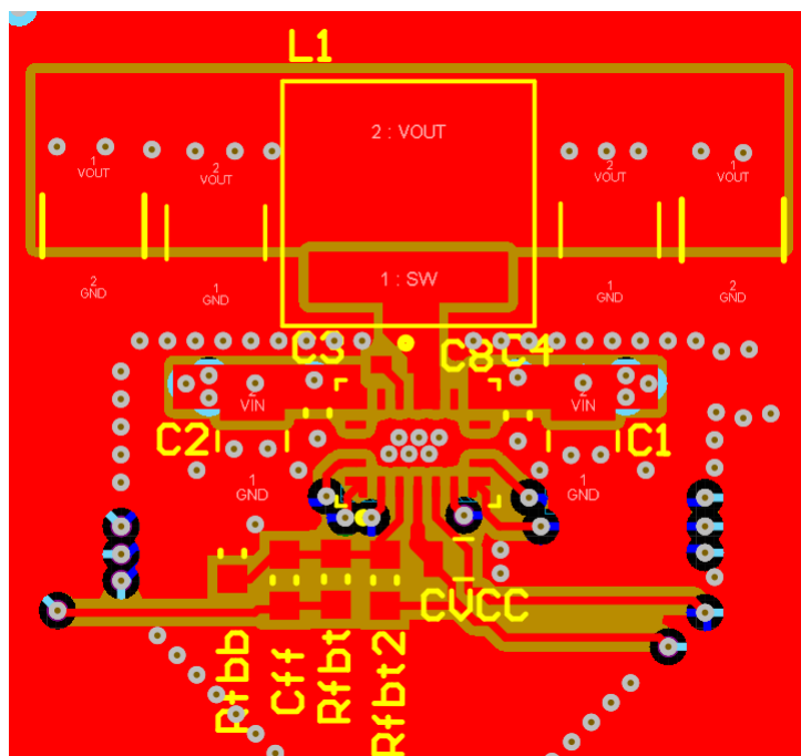
Figure 8-78. Layout Example
