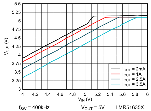
Figure 6-10. 5V Dropout
