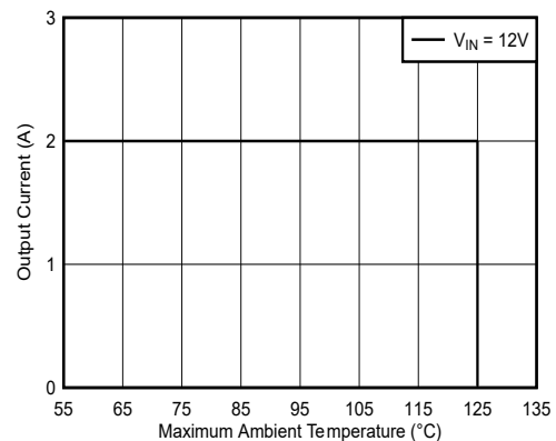
Figure 8-13. Output Current vs Maximum Ambient Temperature
