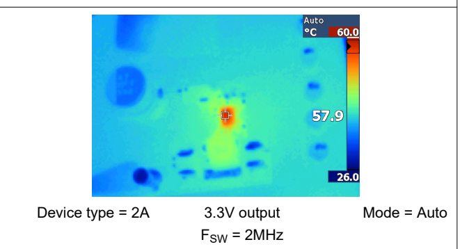
Figure 8-25. Thermal Performance
