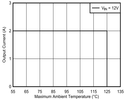
Figure 8-14. Output Current vs Maximum Ambient Temperature
