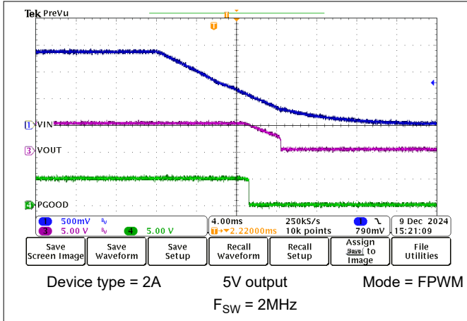
Figure 8-20. Shutdown Operation
