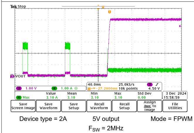
Figure 8-22. Short-Circuit Recovery
