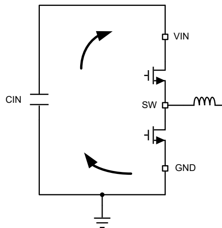
Figure 8-36. Current Loops With Fast Edges
