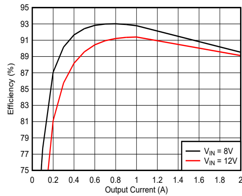
Figure 8-3. Efficiency
