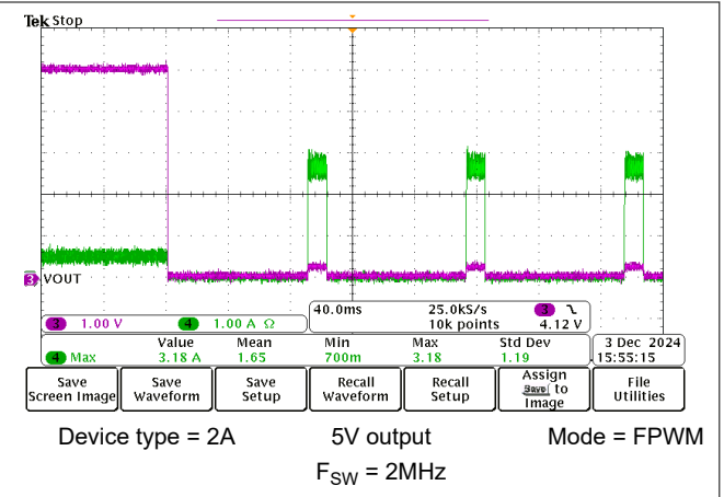
Figure 8-21. Short-Circuit Applied
