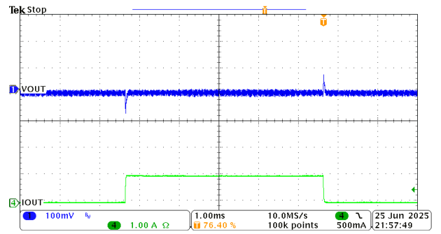
Figure 8-17. 0A to 1A Load Transient
