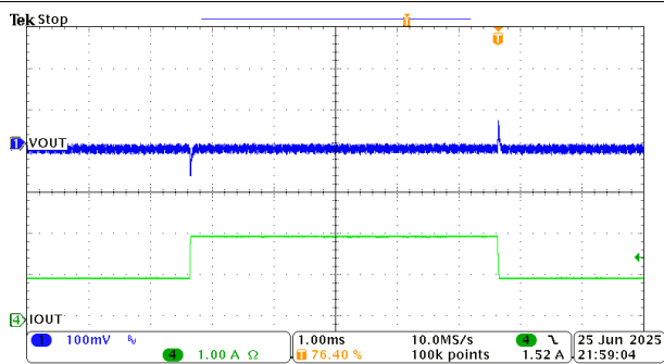
Figure 8-16. 1A to 2A Load Transient
