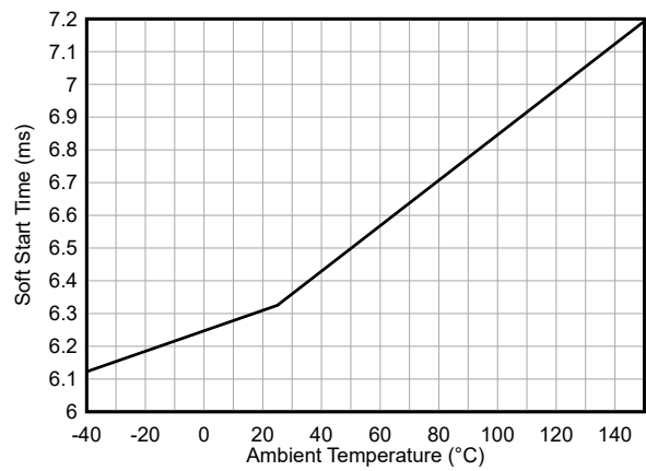
Figure 6-6. Soft-Start Time
