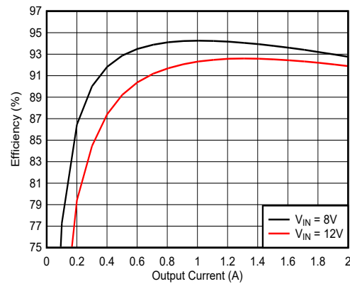
Figure 8-5. Efficiency
