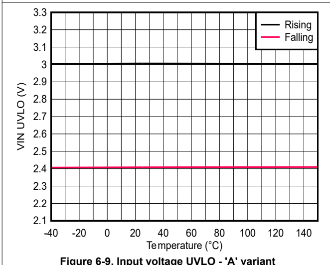
Figure 6-9. Input voltage UVLO - 'A' variant
