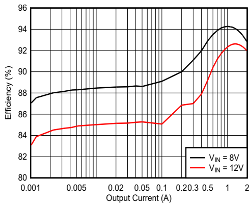
Figure 8-4. Efficiency
