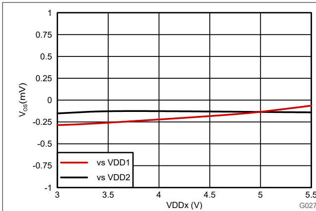
Figure 6-6. Input Offset Voltage vs Supply Voltage
