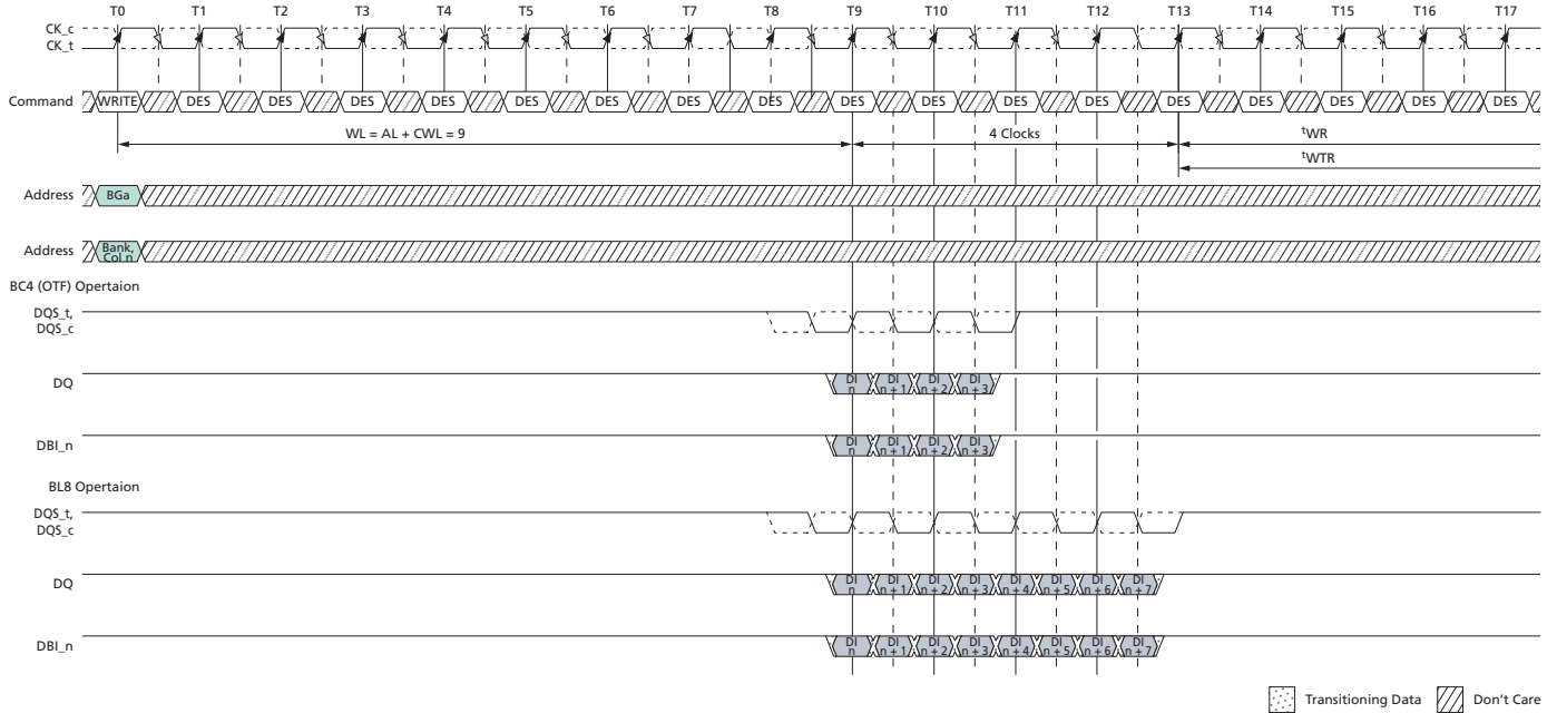
Figure 183: WRITE (BL8/BC4-OTF) with 1 st CK Preamble and DBI
