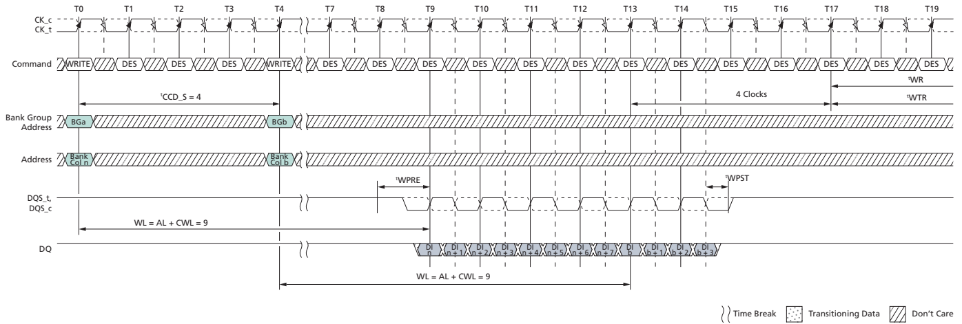
Figure 171: WRITE (BL8) to WRITE (BC4) OTF with 1^t\text{CK} Preamble in Different Bank Group
