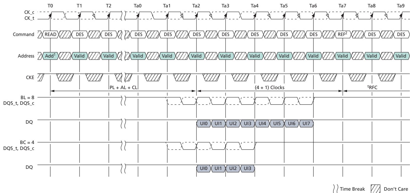
Figure 32: READ-to-REFRESH Timing
