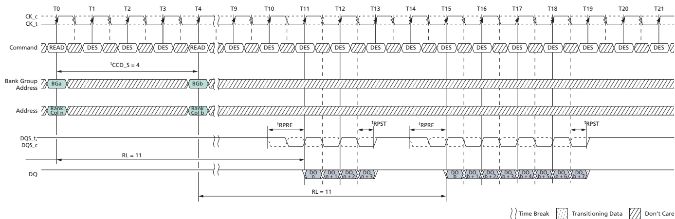
Figure 130: READ (BC4) to READ (BL8) OTF with 1 t CK Preamble in Different Bank Group
