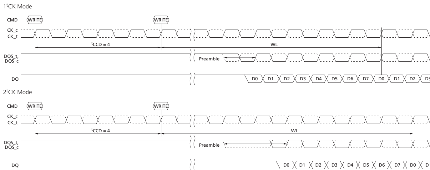
Figure 101: 1 t CK vs. 2 t CK WRITE Preamble Mode, t CCD = 4
