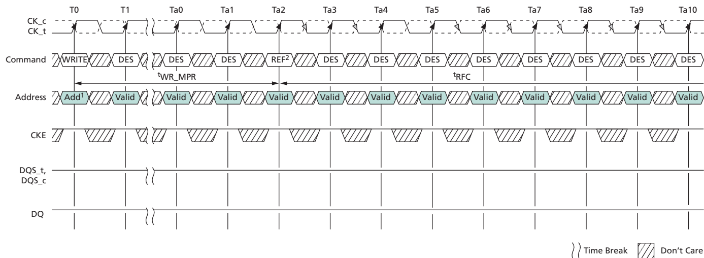
Figure 33: WRITE-to-REFRESH Timing
