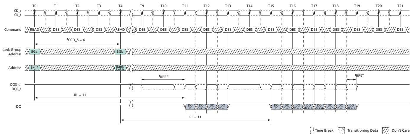
Figure 131: READ (BC4) to READ (BL8) OTF with 2 t CK Preamble in Different Bank Group
