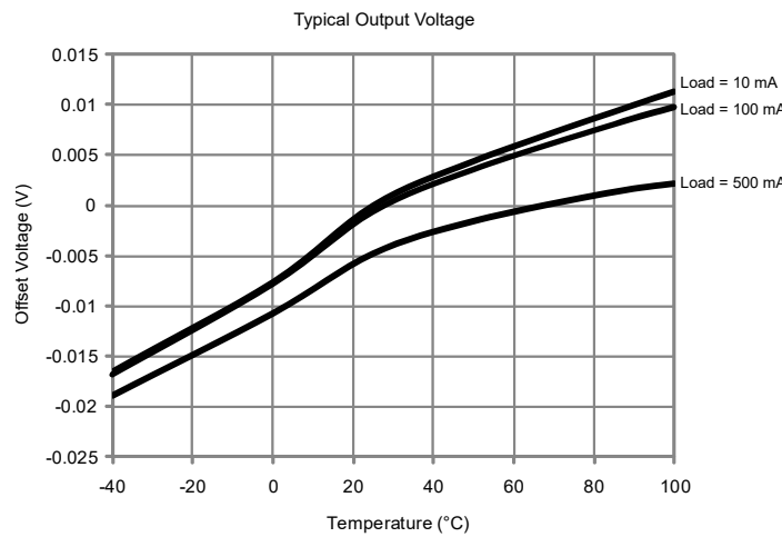
Figure 2-56. Typical Output Voltage
