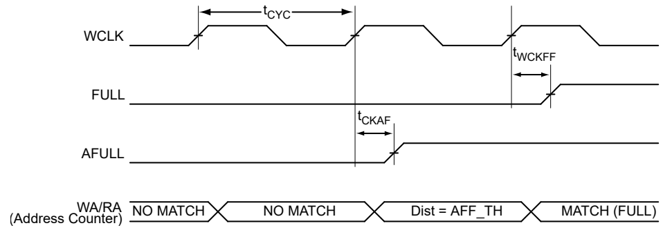
Figure 2-49. FIFO EMPTY Flag and AEMPTY Flag Deassertion
