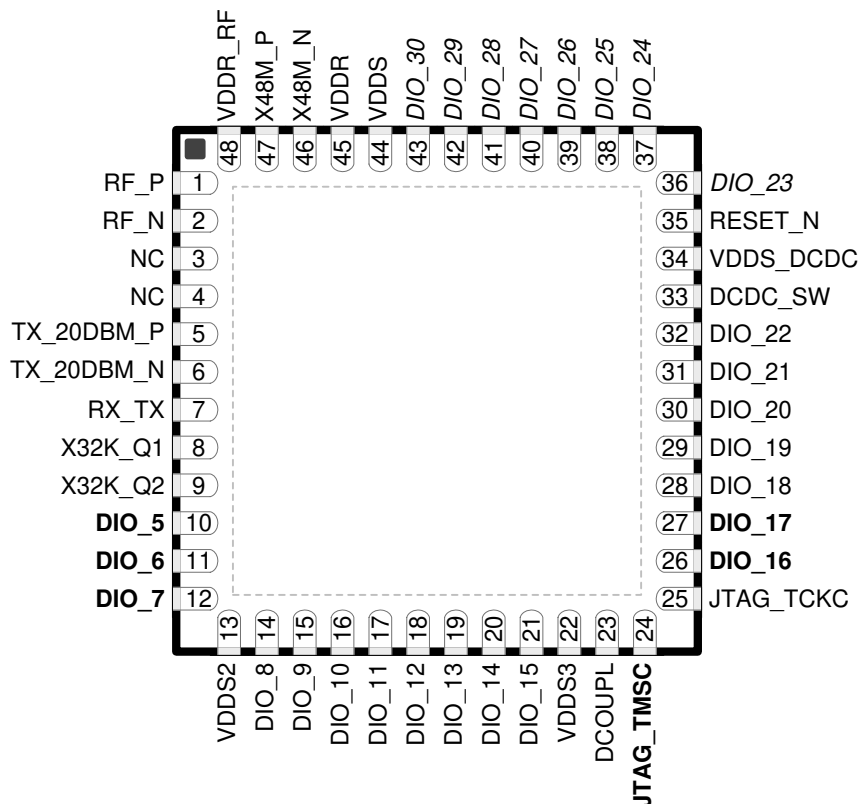
Figure 7-1. RGZ (7-mm x 7-mm) Pinout, 0.5-mm Pitch (Top View)
