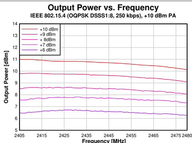
Figure 8-32. Output Power vs. Frequency (250 kbps, +10 dBm PA)
