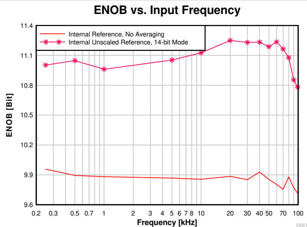
Figure 8-33. ENOB vs. Input Frequency
