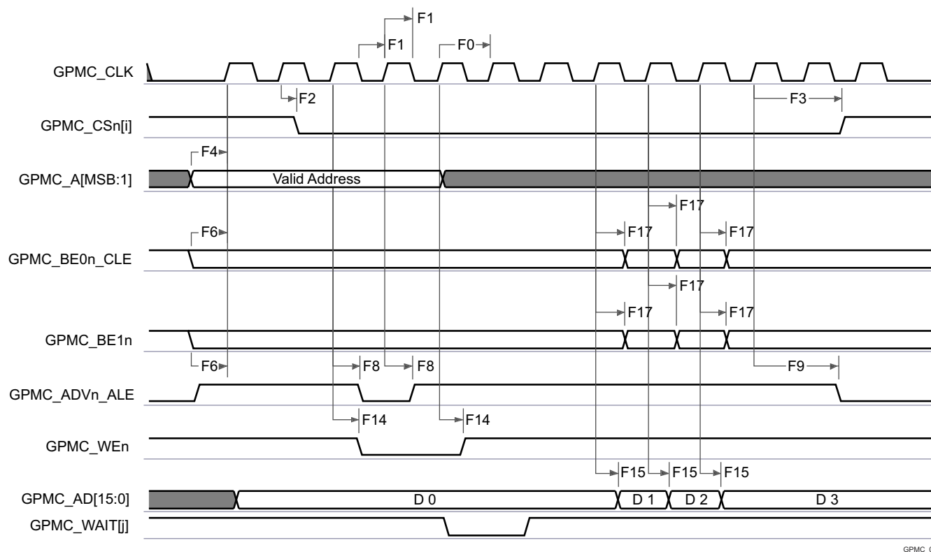
Figure 7-58. GPMC and NOR Flash — Synchronous Burst Read — 4x16-bit (GPMCFCLKDIVIDER = 0)
