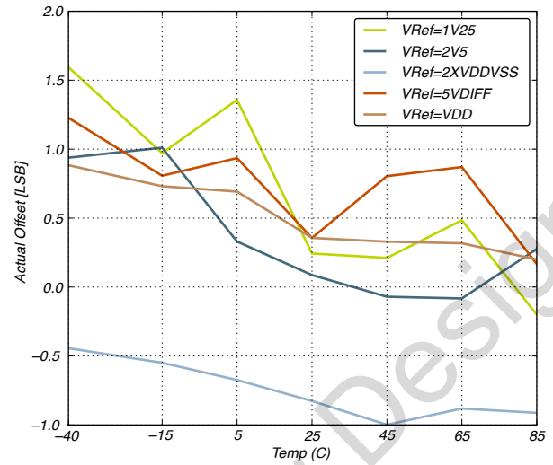
Offset vs Temperature, V_{DD} = 3\text{ V}
