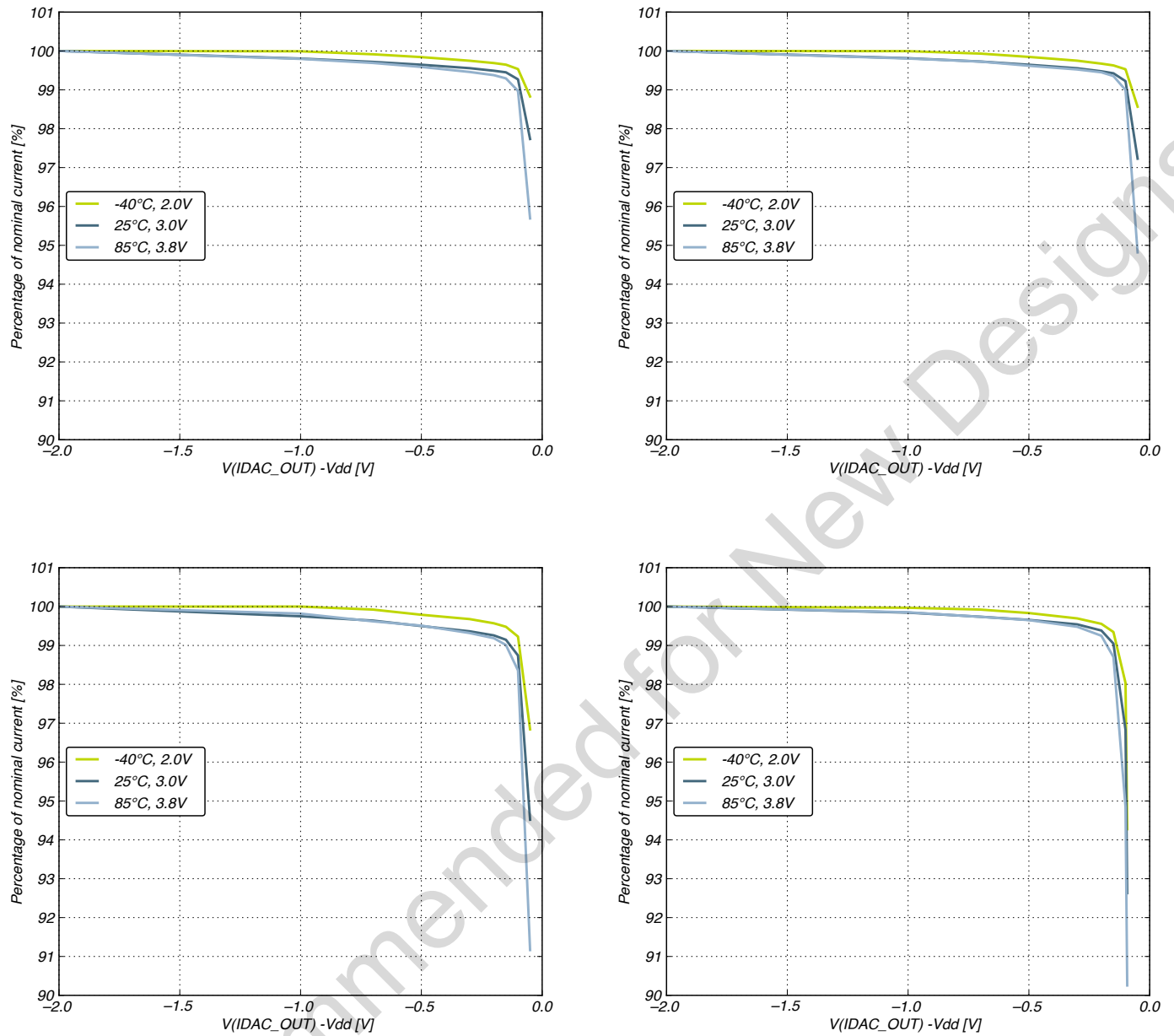
Figure 4.35. IDAC Source Current as a Function of Voltage on IDAC_OUT
