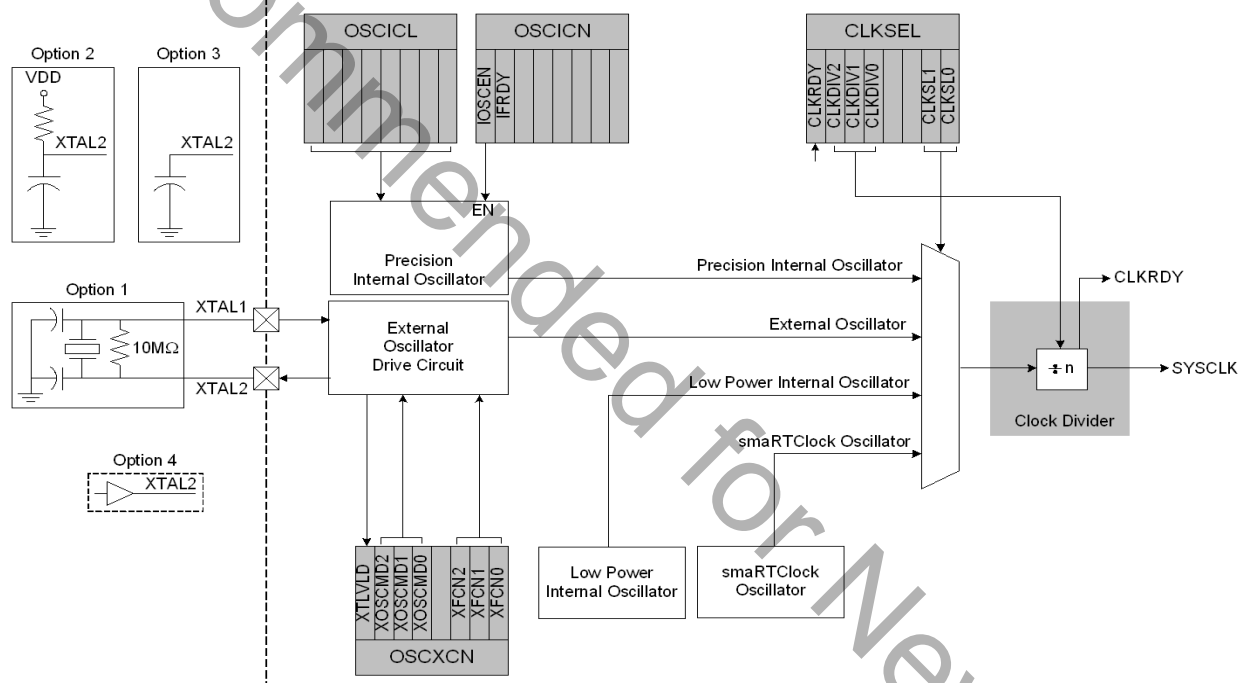
Figure 18.1. Clocking Sources Block Diagram
