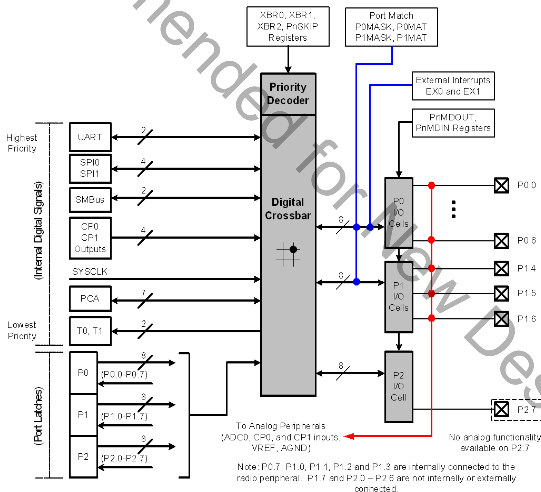
Figure 20.1. Port I/O Functional Block Diagram
