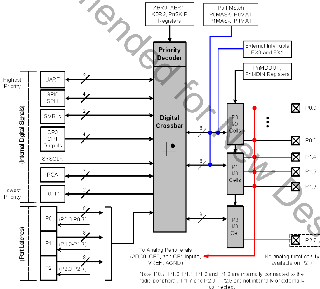
Figure 1.4. Port I/O Functional Block Diagram
