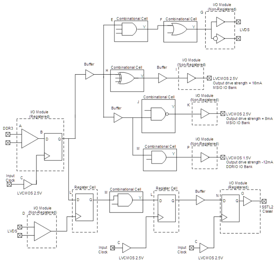
FIGURE 3-2: TIMING MODEL
