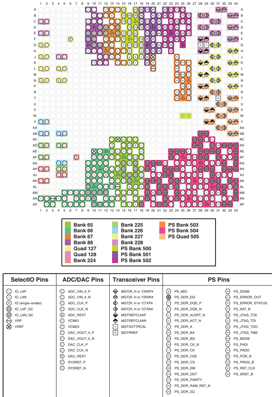
Figure 4-65: FFVE1156 and FSVE1156 Packages—XCZU65DR I/O Bank Diagram
