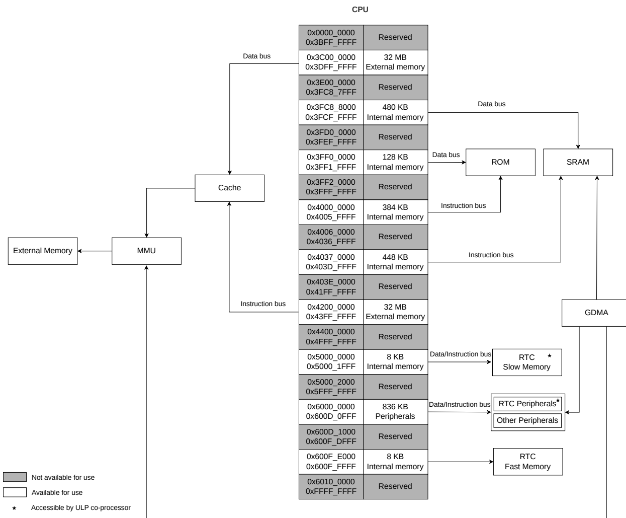
Figure 4-1. Address Mapping Structure
