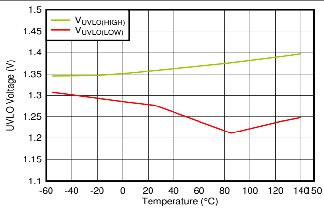
Figure 6-40. UVLO Rising and Falling Threshold vs Temperature
