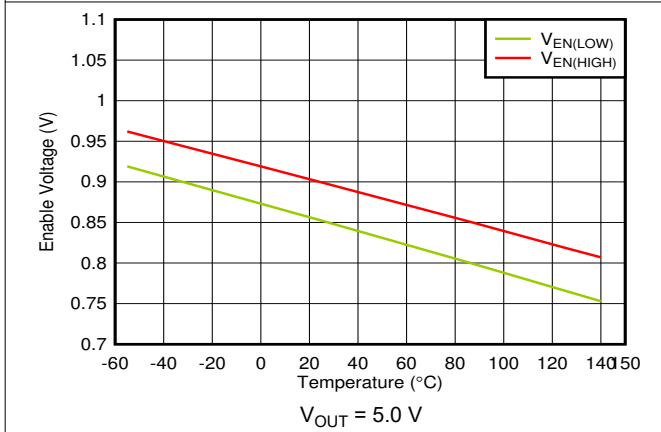
Figure 6-39. EN High and Low Threshold vs Temperature
