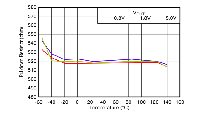
Figure 6-42. Smart Enable Pulldown Resistor vs Temperature and V_{OUT}
