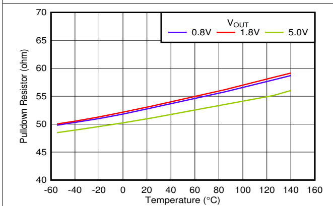
Figure 6-41. Pulldown Resistor vs Temperature and V_{OUT}
