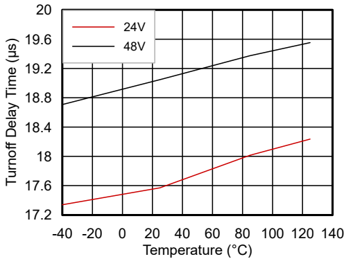
Figure 6-5. Turn-off Delay Time ( t_{DF} ) vs Temperature vs VS Voltage
