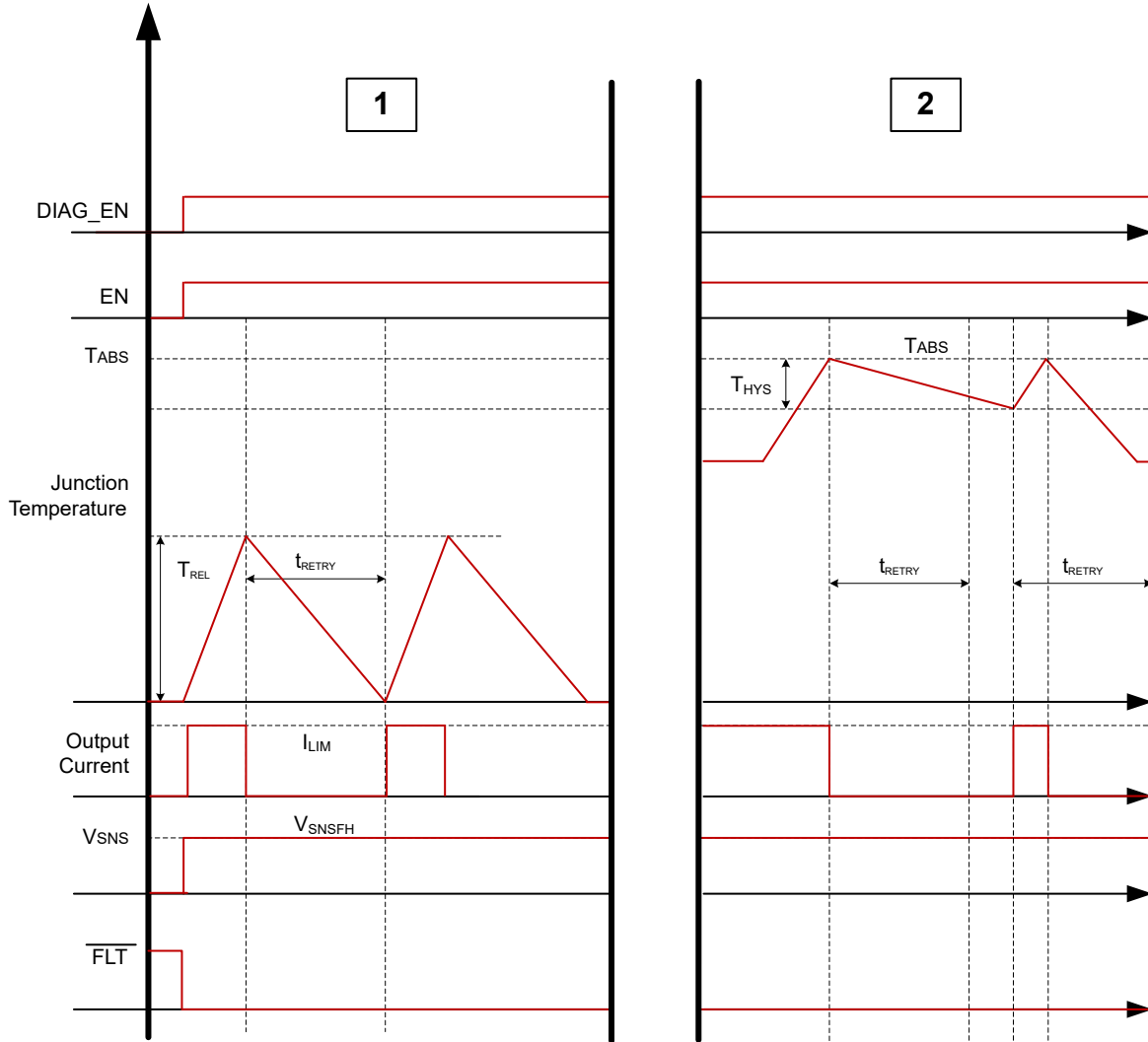
Figure 8-16. Thermal Behavior
