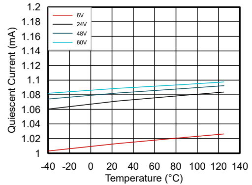
Figure 6-2. Quiescent Current ( I_{Q, vs} ) From VS Input Supply vs Temperature vs VS Voltage V_{EN} = 5\text{ V} V_{DIAG\_EN} = 0\text{ V}
