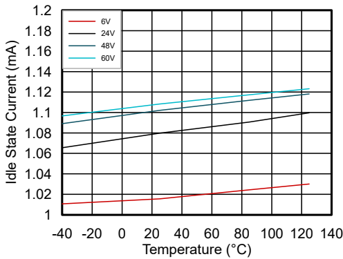
Figure 6-3. Idle State Current ( I_{IDLE, vs} ) From VS Input Supply vs Temperature vs VS Voltage V_{EN} = 0\text{ V} V_{DIAG\_EN} = 0\text{ V}
