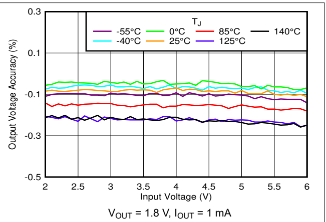
Figure 6-26. Output Accuracy vs V_{IN} and Temperature
