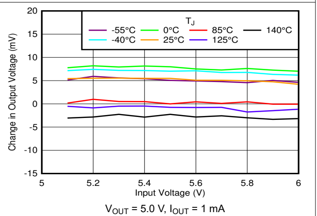
Figure 6-28. Line Regulation vs V_{IN} and Temperature
