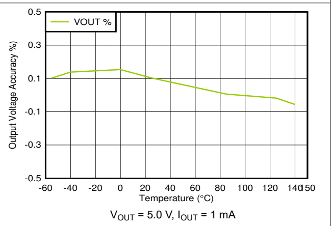
Figure 6-30. Output Accuracy vs Temperature
