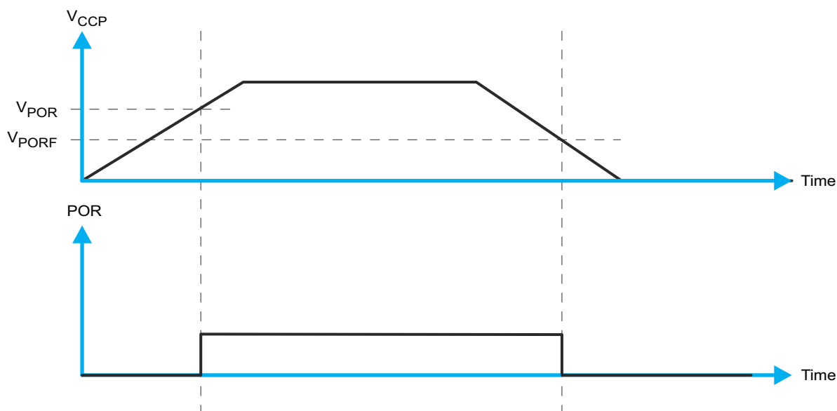
Figure 8-8. V_{POR}
