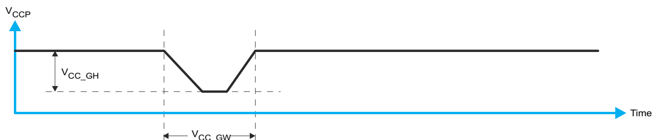
Figure 8-7. Glitch Width and Glitch Height
