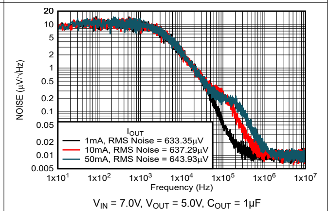
Figure 5-42. Noise vs Load Current
