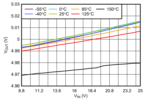
Figure 5-2. V_{OUT} vs V_{IN}
