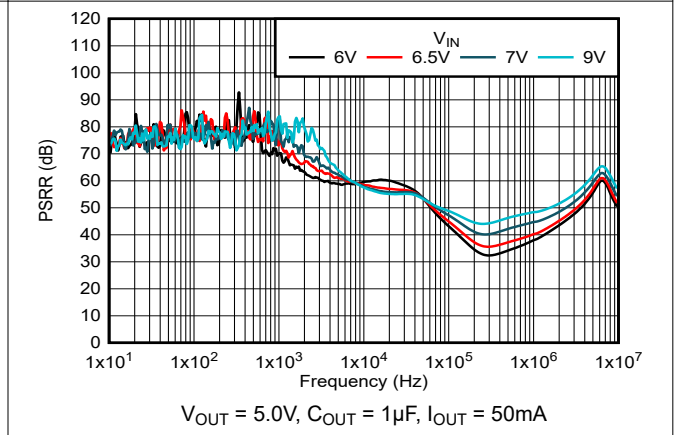
Figure 5-40. PSRR vs Input Supply
