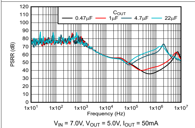
Figure 5-41. PSRR vs Output Capacitor
