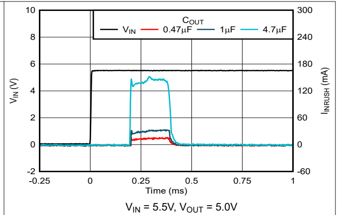
Figure 5-38. Inrush Current vs Output Capacitor
