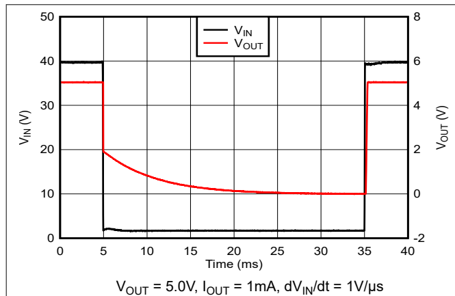
Figure 7-16. Brownout Transient (40V to 1.7V)
