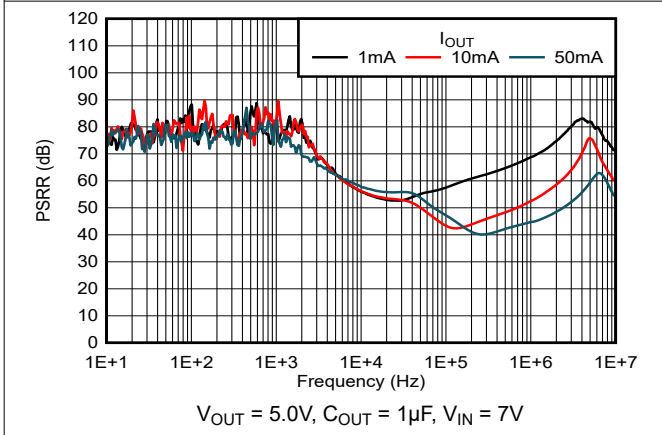
Figure 5-39. PSRR vs Load Current
