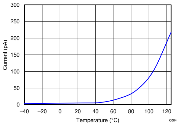
Figure 5-5. Leakage vs Temperature
