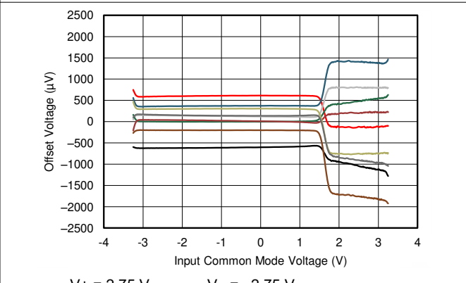
Figure 8-4. Offset Voltage vs Common-Mode Voltage
