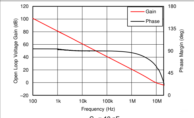
Figure 8-6. Open-Loop Gain and Phase vs Frequency
