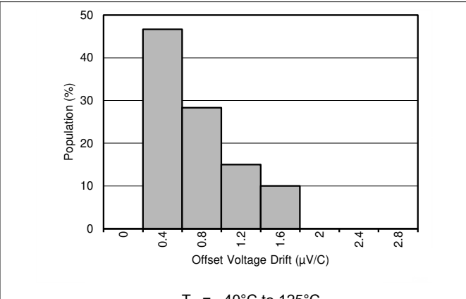
Figure 8-2. Offset Voltage Drift Distribution
