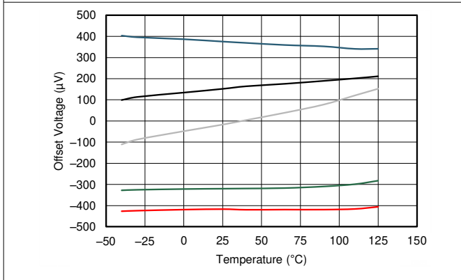
Figure 8-3. Offset Voltage vs Temperature
