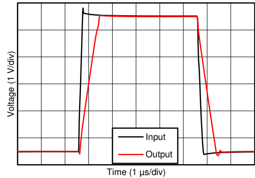
Figure 8-26. Overload Recovery
