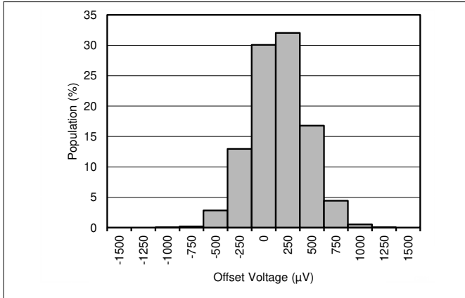
Figure 8-1. Offset Voltage Production Distribution
