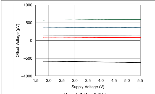
Figure 8-5. Offset Voltage vs Power Supply
