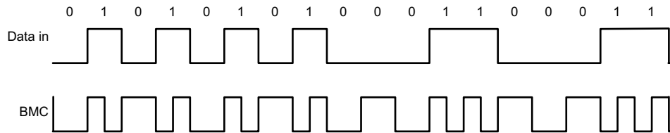
Figure 8-6. Biphas Mark Coding Example
