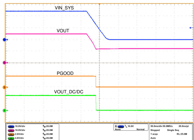
Figure 9-8. Power-Down Response
