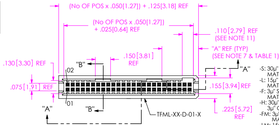
FIG 1 -01: THROUGH HOLE
