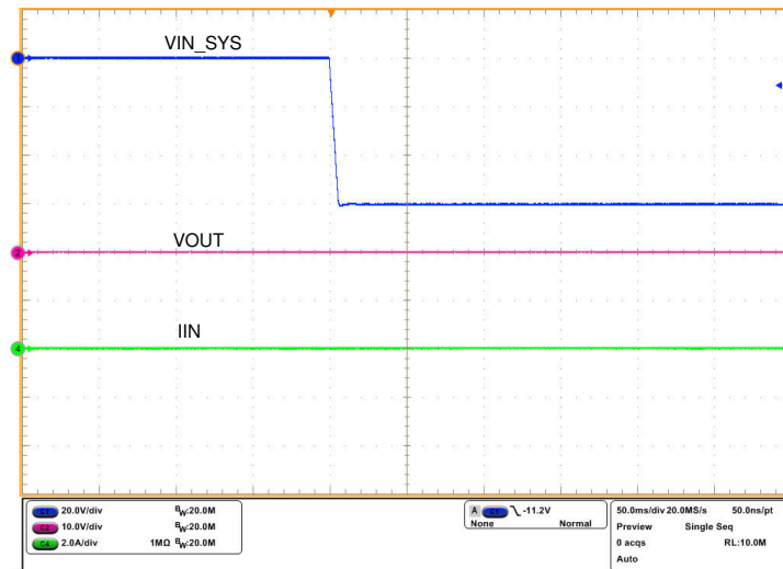
Figure 8-9. Input Reverse Polarity Response at -60\text{-V} Input
