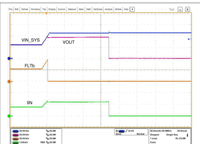
Figure 8-6. Overvoltage Clamp Response With TPS26635 R_{LOAD} = 30 \Omega , FLT connected to VOUT
