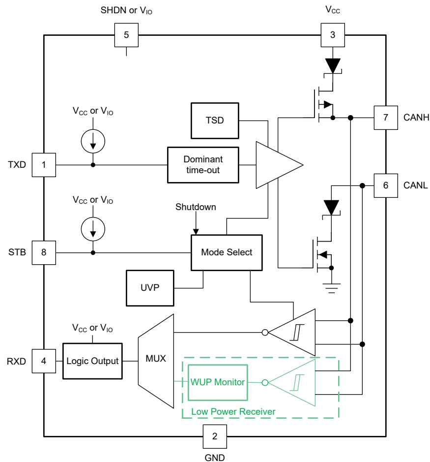
Figure 7-1. Block Diagram
