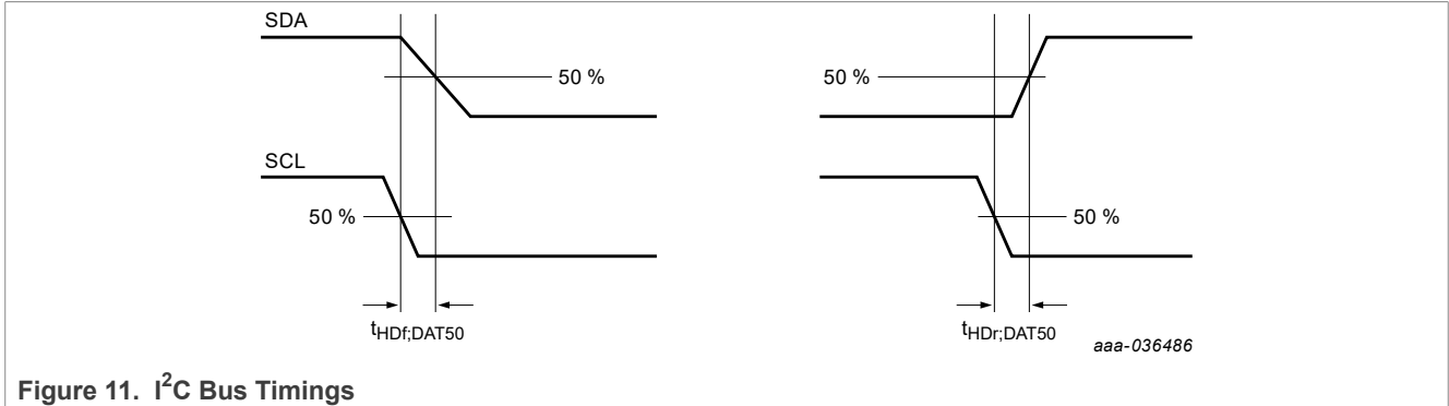
Figure 11. I 2 C Bus Timings
