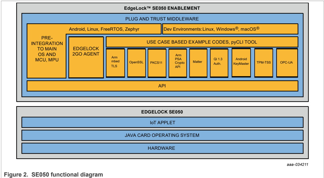
Figure 2. SE050 functional diagram
