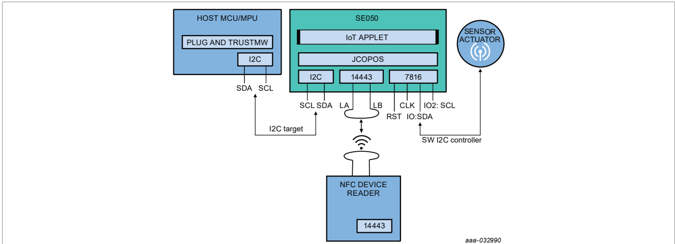
Figure 1. SE050 solution block diagram
