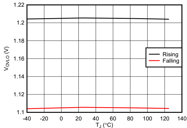
Figure 6-3. OVLO Pin Threshold vs Temperature
