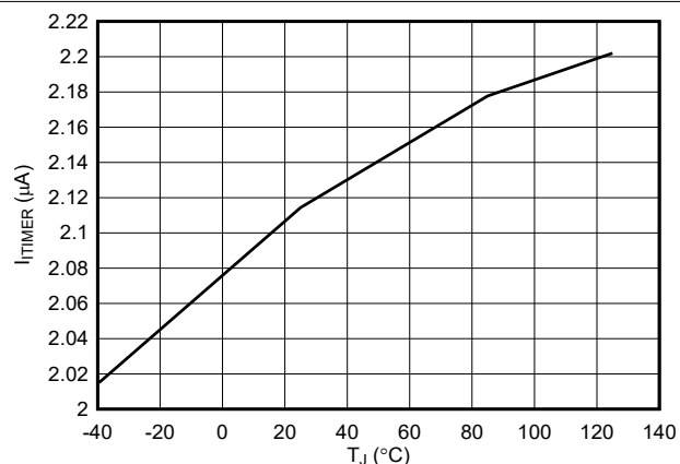
Figure 6-17. ITIMER Discharge Current vs Temperature
