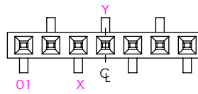
ODD POSITIONS X = ((\text{NO OF POS} - 1) / 2), Y = X+1
