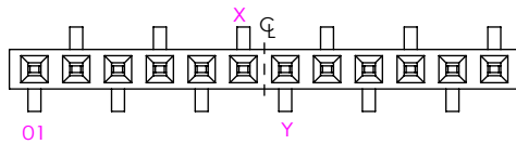
EVEN POSITIONS X = (\text{NO OF POS} / 2), Y = X+1
