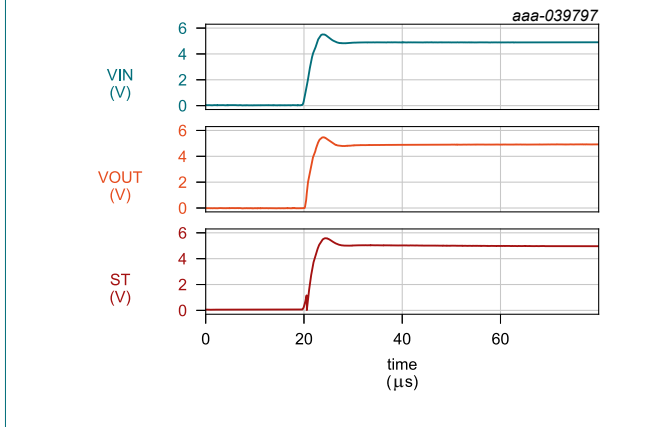
V IN = 5 V; V EN = 0 V; C L = 100 nF; R L = 1 kΩ
